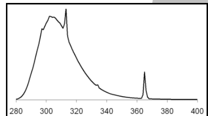
UVB-Spectrum
