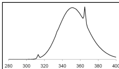
UVA-Spectrum
